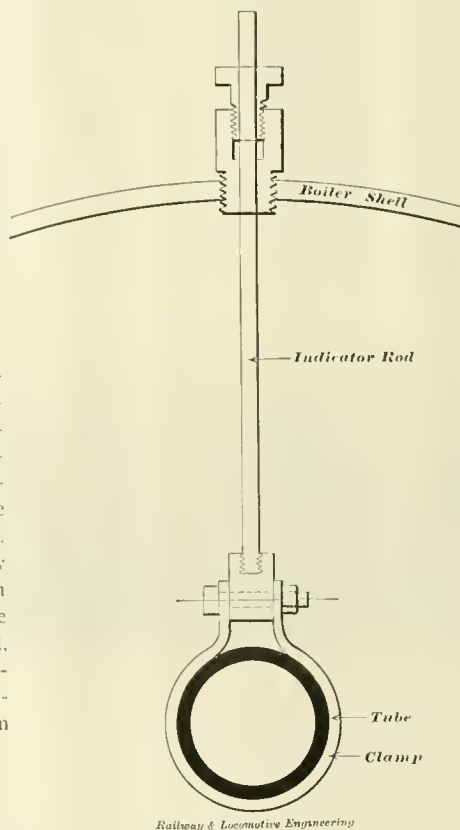
Railway & Locomotive Engineering TEST FOR TUBE VIBRATION.
